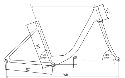
TOUR - CITY: Aluminum alloy monotube 26"
